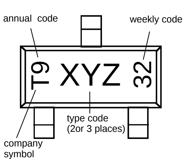
SOT23 (Transistor)
