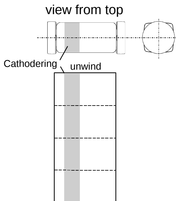
SOD80 – QuadroMELF
