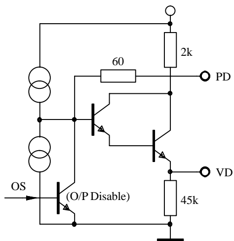
Figure 9. Loop amplifier
