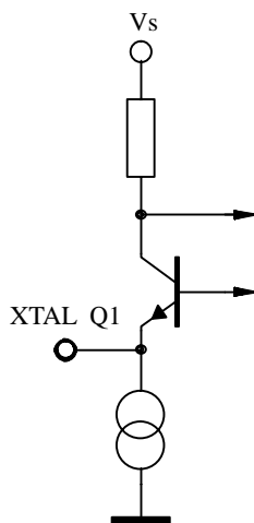
Figure 13. Reference oscillator
