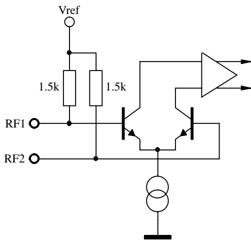
Figure 8. RF input
