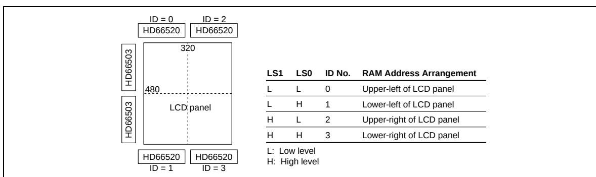
Figure 2 LS Pins and Address Assignment
