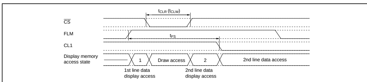
Figure 35 Chip Select Low Level Width
