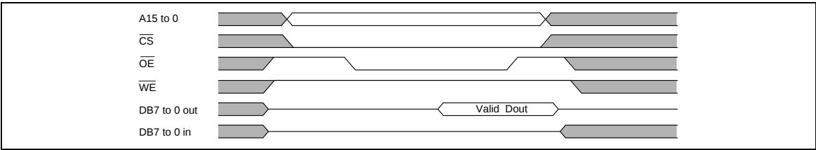
Figure 24 Read Cycle
