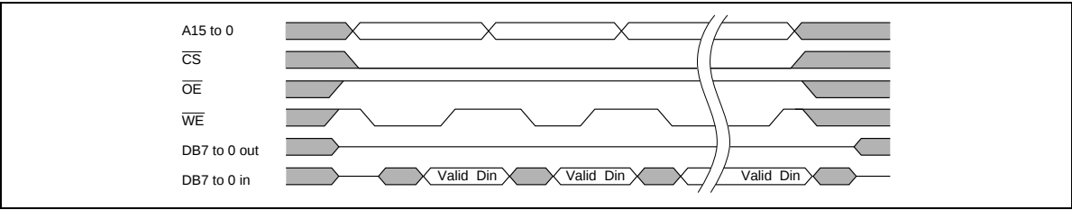
Figure 27 Burst Write Cycle
