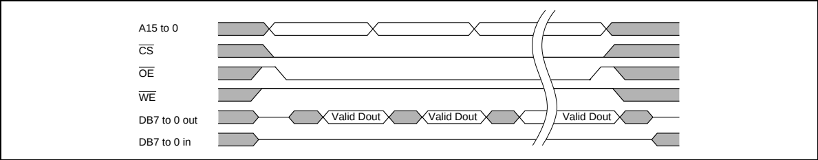
Figure 26 Burst Read Cycle
