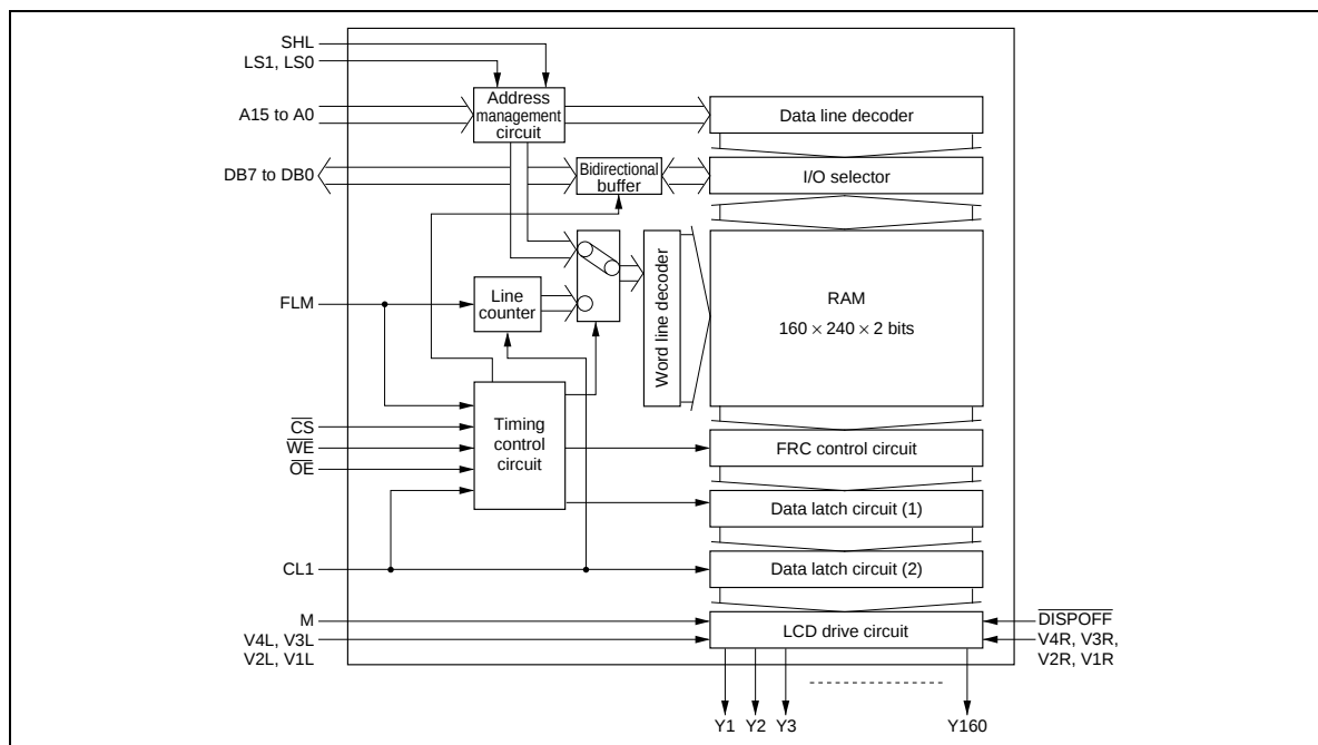
Figure 4 Block Diagram
