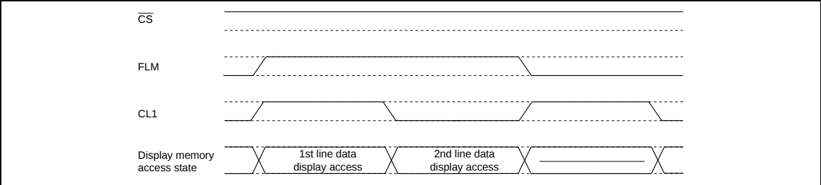
Figure 31 First Line Data Transfer
