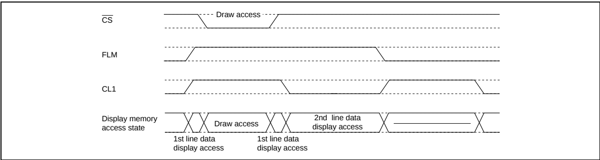
Figure 32 Draw Access (3)
