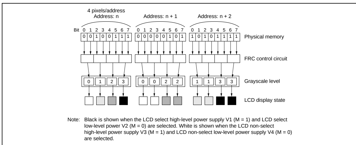
Figure 5 Packed Pixel System
