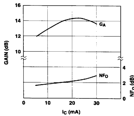
Figure 2. Optimum Noise Figure and Associated Gain vs. Collector Current and Frequency. V_{CE} = 8\text{ V} , f = 2.0\text{ GHz} .
