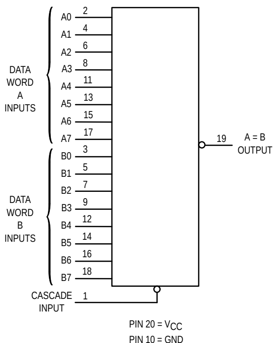
LOGIC DIAGRAM
